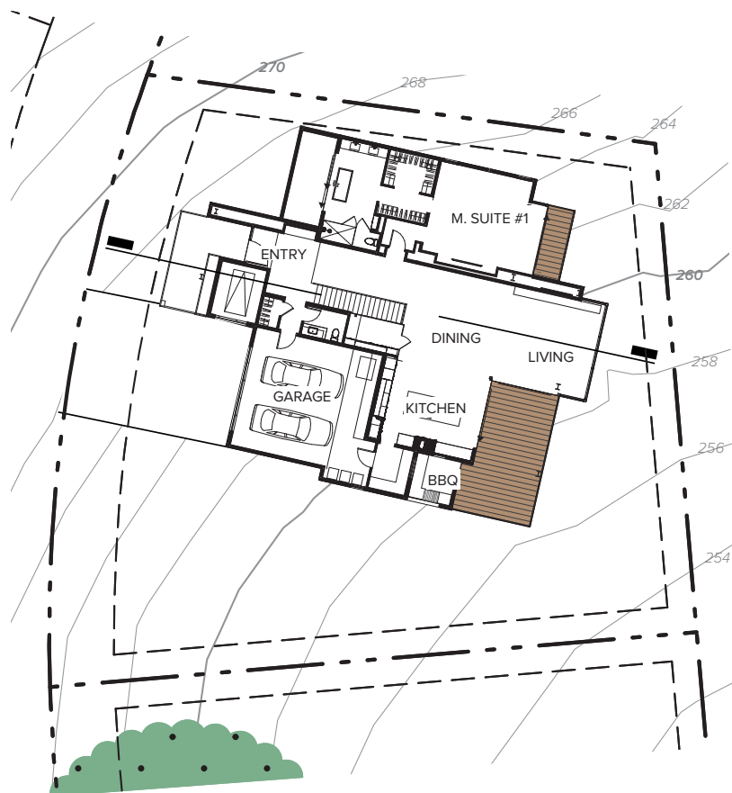
ENTRY LEVEL
