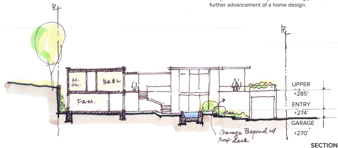
SECTION
