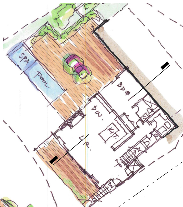
MIDDLE LEVEL
