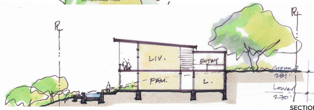
SECTION
