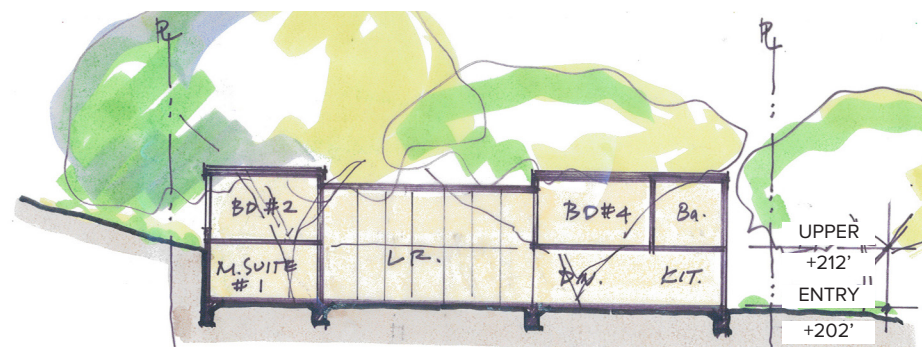
SECTION
