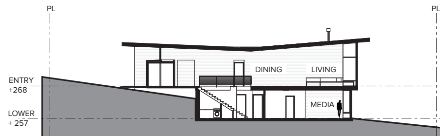
SECTION
