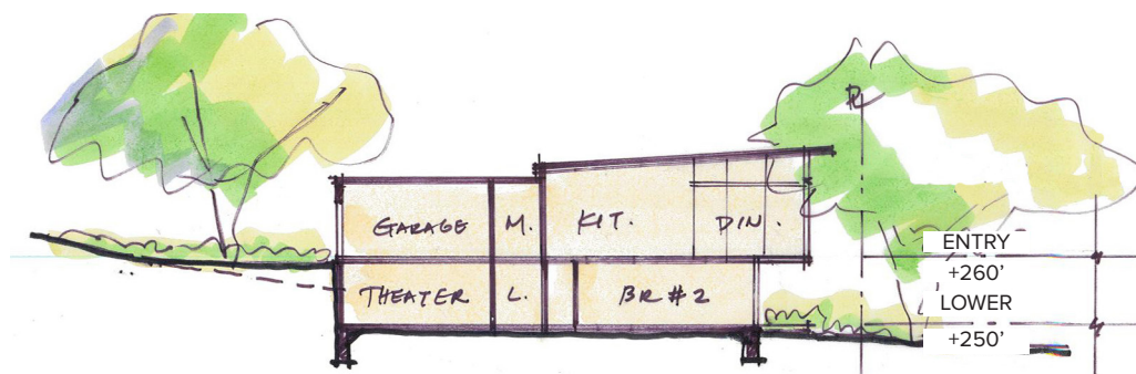
SECTION
