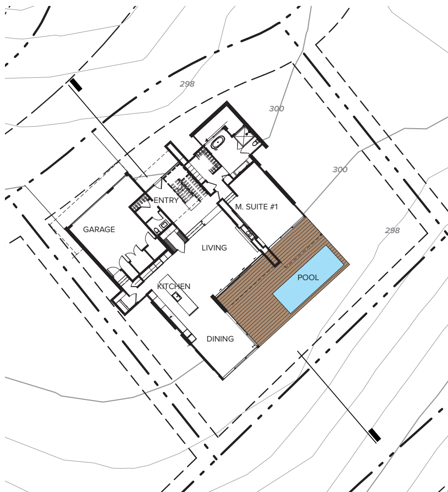
ENTRY LEVEL
