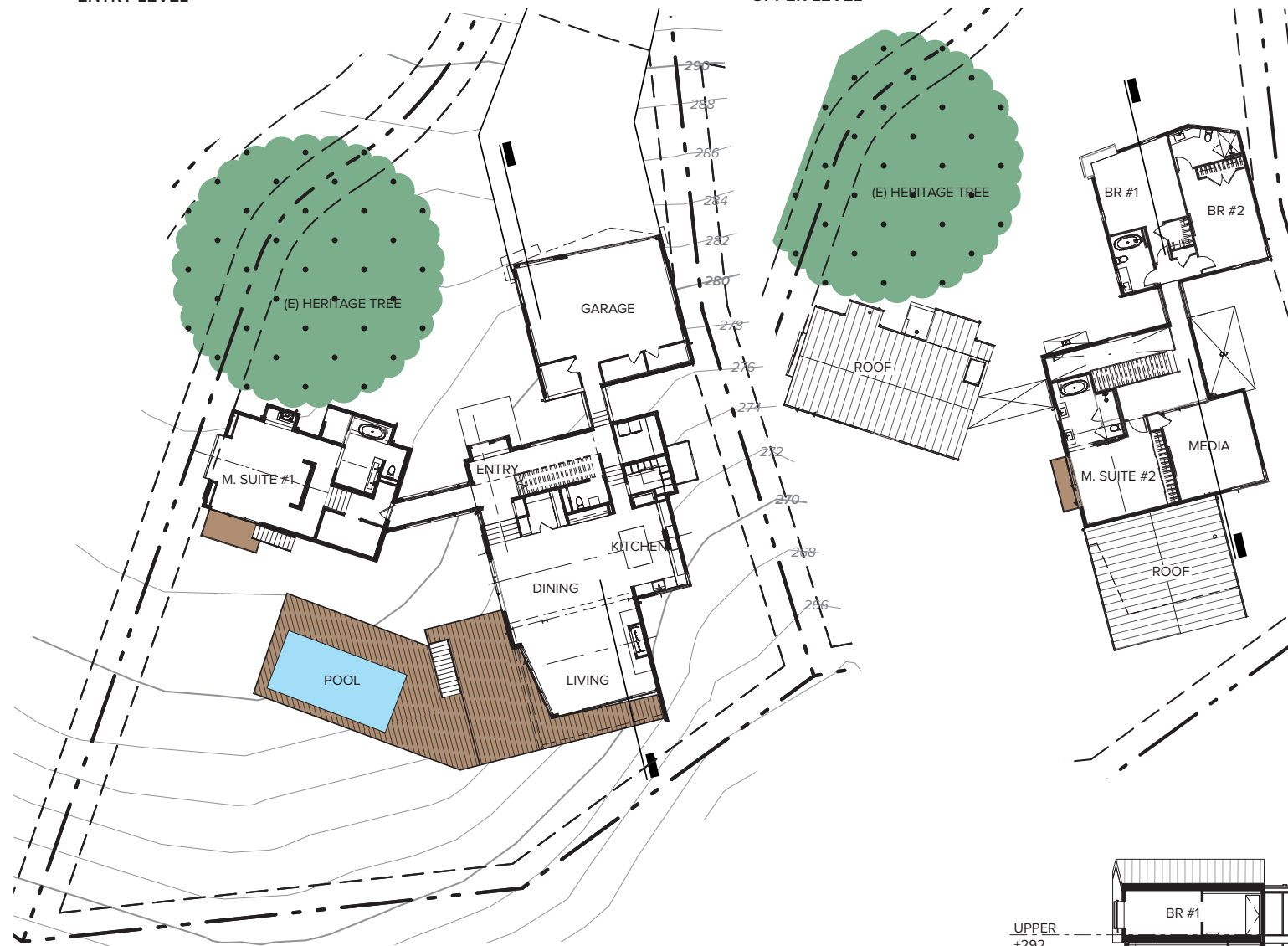
UPPER LEVEL
