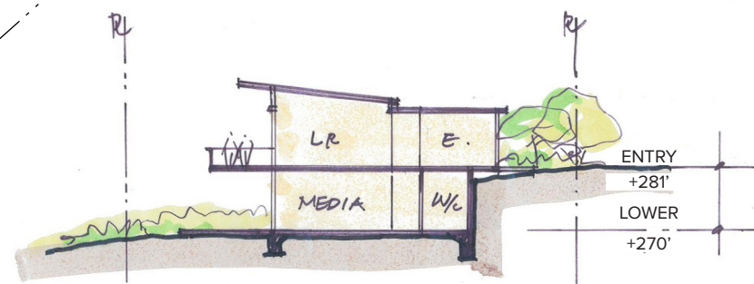
SECTION
